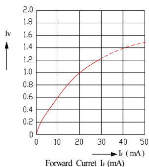
FIG.3 RELATIVE LUMINOUS INTENSITY VS. FORWARD CURRENT
