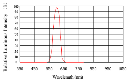
FIG.1 RELATIVE LUMINOUS INTENSITY
