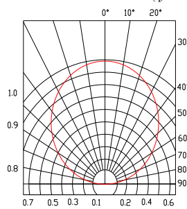
FIG.5 RADIATION DIAGRAM
