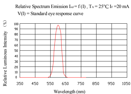
FIG.1 RELATIVE LUMINOUS INTENSITY
