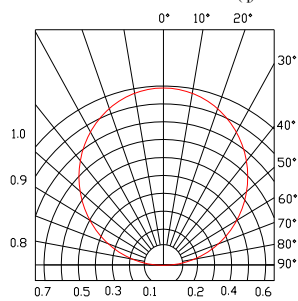
FIG.5 RADIATION DIAGRAM
