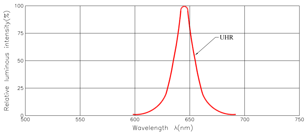
Spectrum Distribution
