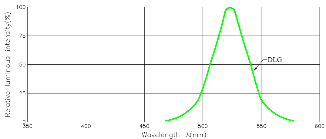
Spectrum Distribution
