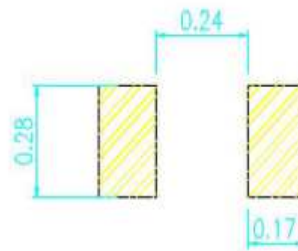
Soldering PAD
