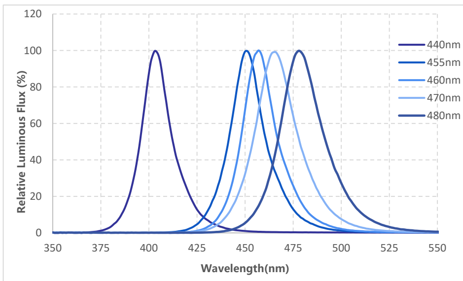
Fig 1. Relative Spectral Luminous Flux Distribution for Dominant Wavelength 440-480nm, IF=700mA, Ta = 25°C, RH60%
