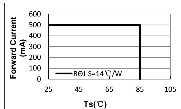
Fig.6- Ts Temperature Vs. Forward Current
