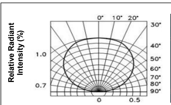
Fig.5- Radiation diagram
