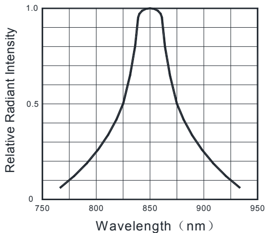
Fig.5 Spectral Distribution
