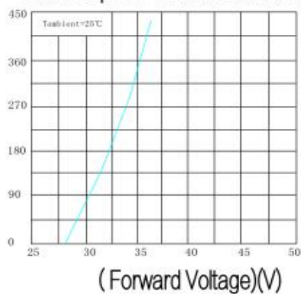
Volt-Ampere Characteristics
