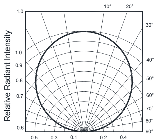
Fig.6 Radiant Diagram
