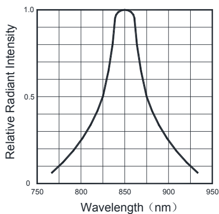
Fig.5 Spectral Distribution
