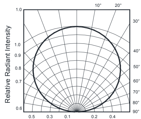
Fig.6 Radiant Diagram
