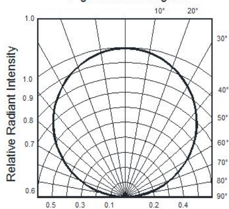
Fig.6 Radiant Diagram
