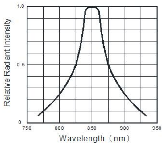
Fig.5 Spectral Distribution
