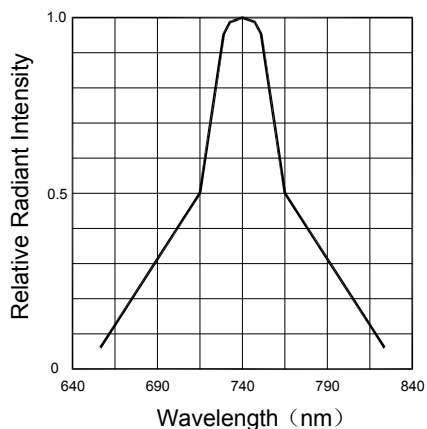
Fig.5 Spectral Distribution
