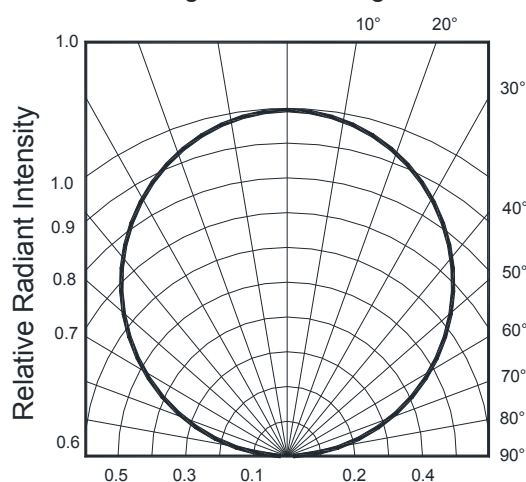
Fig.6 Radiant Diagram
