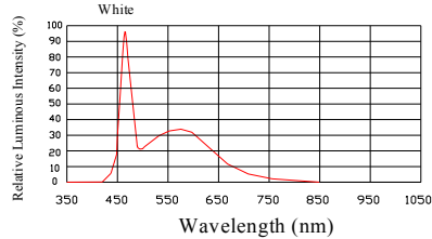
FIG.1 RELATIVE LUMINOUS INTENSITY
