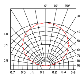
FIG.5 RADIATION DIAGRAM
