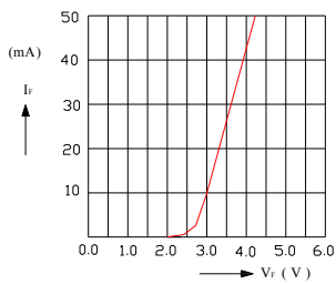
FIG.2 FORWARD CURRENT VS. FORWARD VOLTAGE
