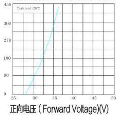
伏安特性 Volt-Ampere Characteristics
