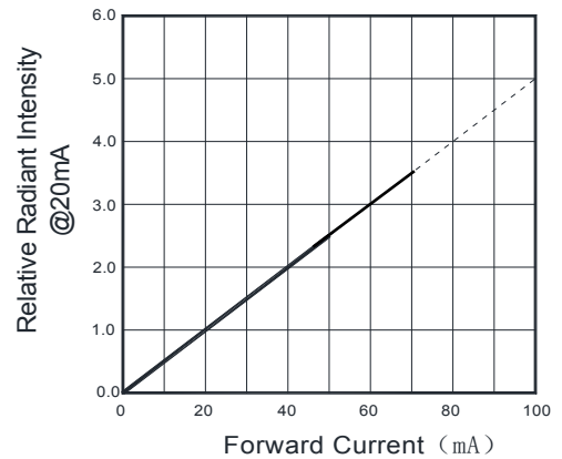
Fig.2 Relative Radiant Intensity Vs Forward Current
