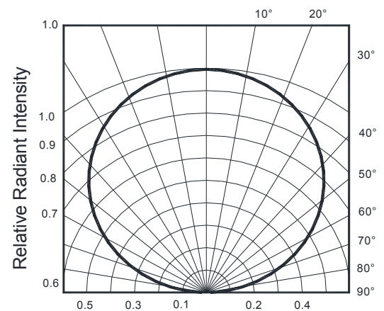
Fig.6 Radiant Diagram
