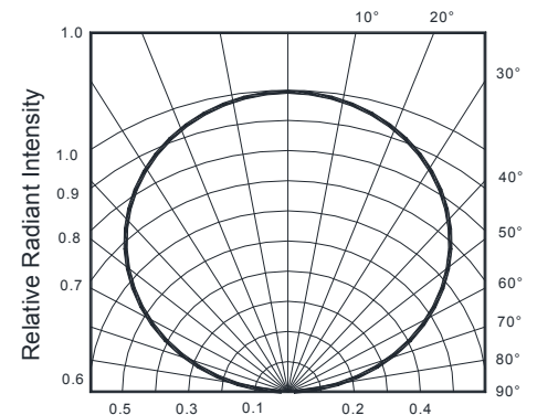
Fig.6 Radiant Diagram
