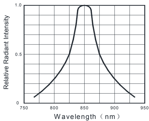
Fig.5 Spectral Distribution
