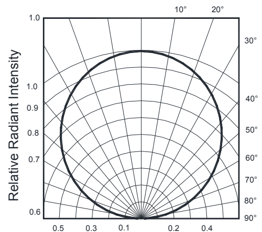
Fig.6 Radiant Diagram
