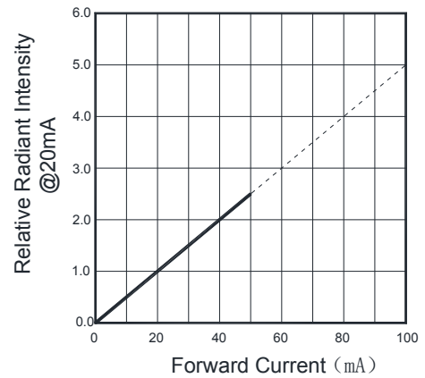
Fig.2 Relative Radiant Intensity Vs Forward Current
