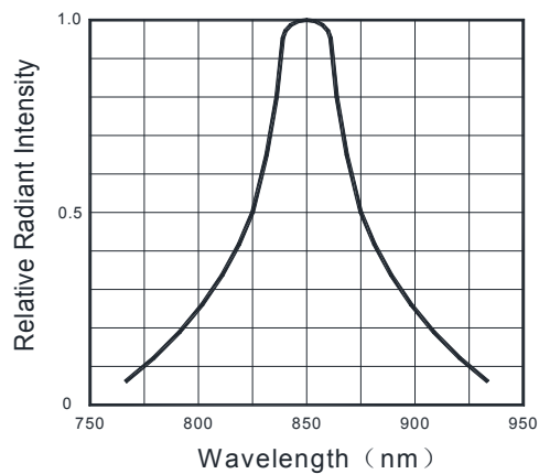
Fig.5 Spectral Distribution
