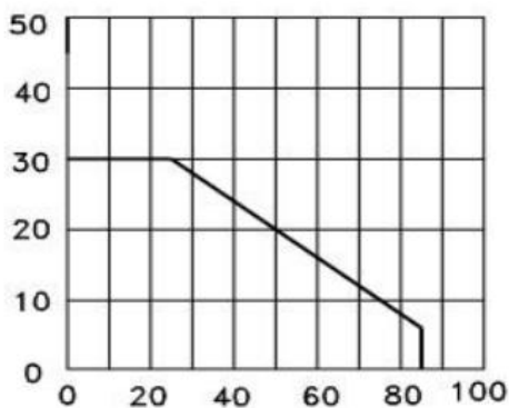
Ambient Temperature vs. Forward Current
