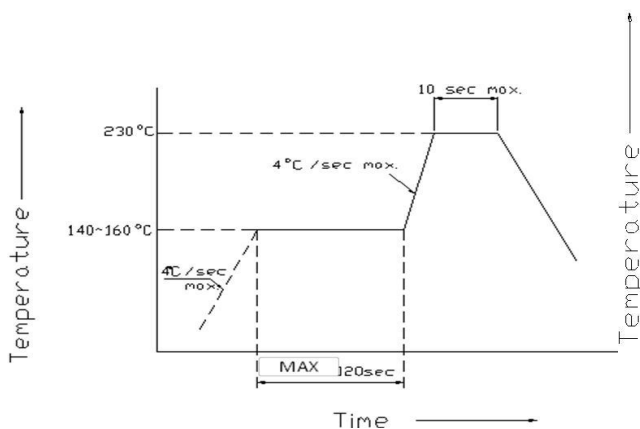
(Lead Solder)
