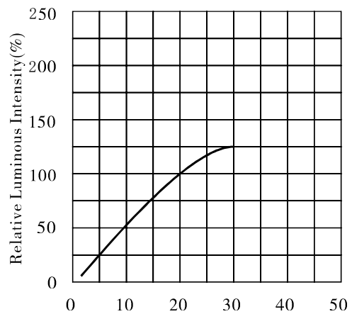
Forward Current I_F (mA) Directive Characteristics Ambient Temperature T_a (°C)
