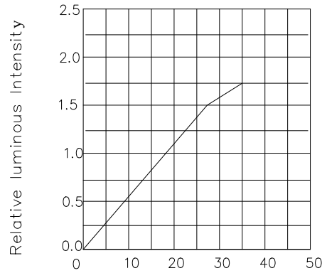
Forward Current(mA)
