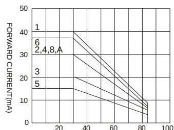
FORWARD CURRENT VS. AMBIENT TEMPERATURE
