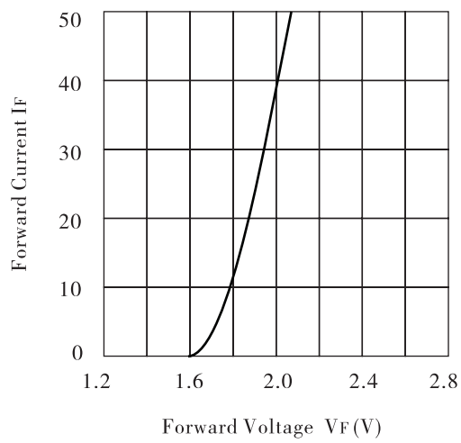
Typical Electro-Optical characteristic curves ( T_a=25^{\circ}\text{C} )
