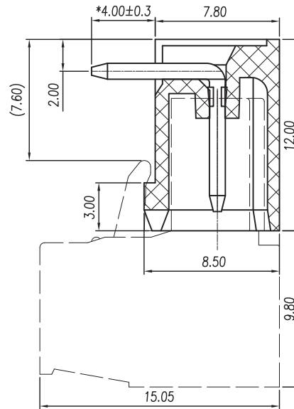
SECTION: A-A
