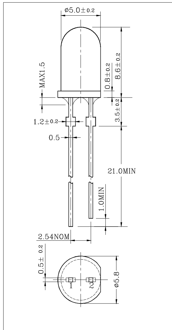
W85I5315-C(B) PIN Connections
