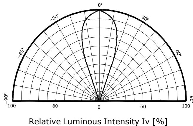
Fig.5 Radiation Characteristics
