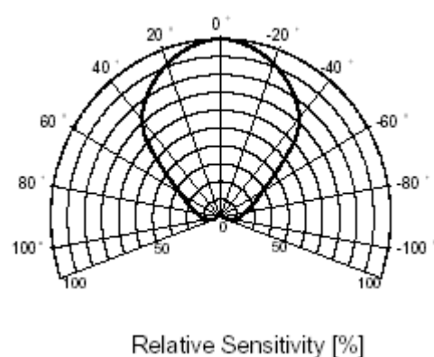
[ Fig.7 ] Directivity (Horizontal)
