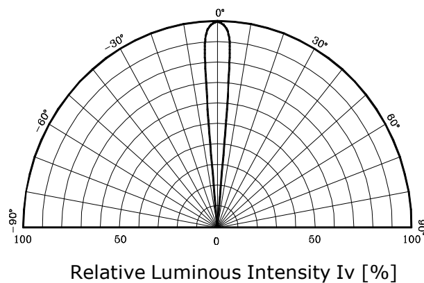
Fig.5 Radiation Characteristics
