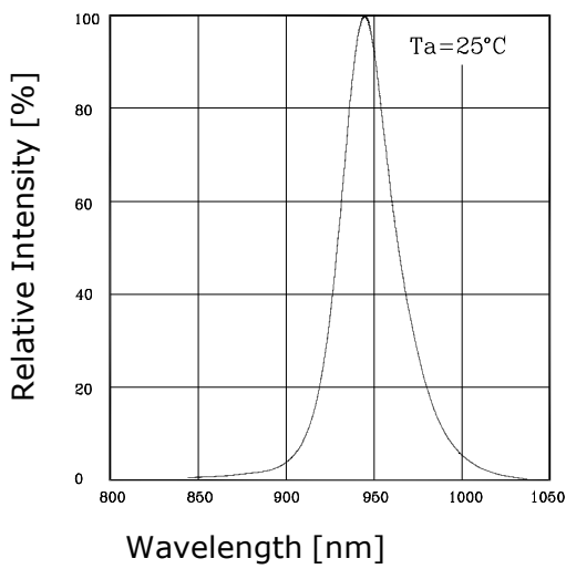
Fig.3 Spectrum Distribution
