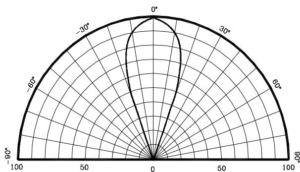
Fig.5 Radiation Characteristics
