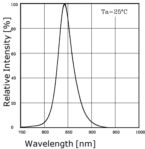
Fig.3 Spectrum
