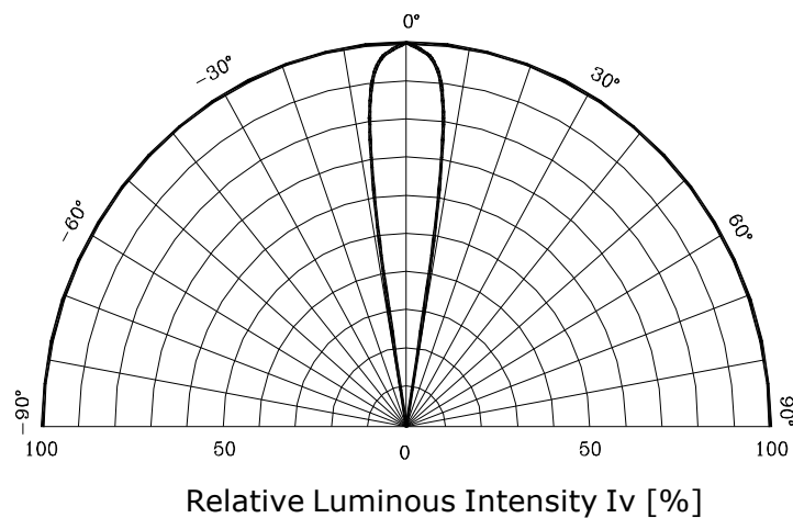
Fig.5 Radiation Characteristics
