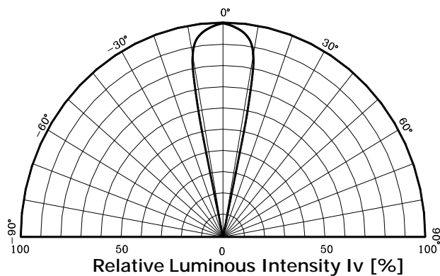
Fig.5 Radiation Characteristics
