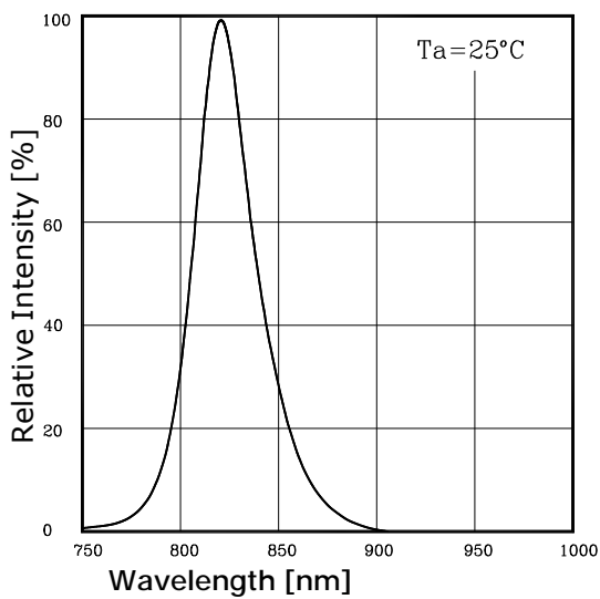
Fig.3 Spectrum Distribution
