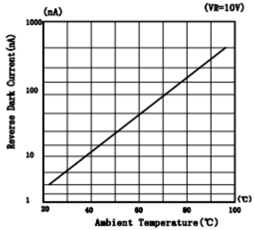
Reverse Light Current vs. Ee
