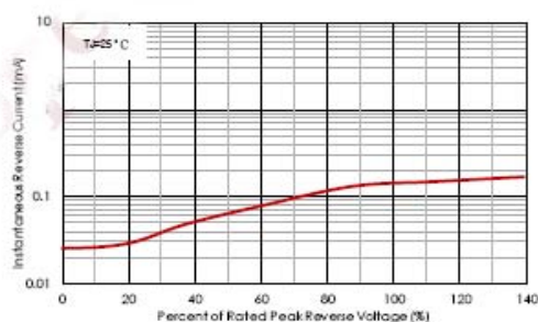
Fig 4 Typical Reverse Characteristics
