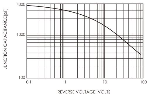
FIG.5-TYPICAL JUNCTION CAPACITANCE
