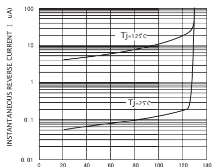
FIG.5-TYPICAL REVERSE CHARACTERISTICS
