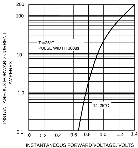
FIG.3-TYPICAL FORWARD CHARACTERISTICS
