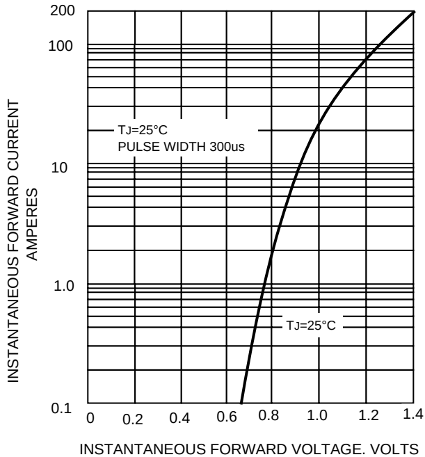
FIG.2-TYPICAL FORWARD CHARACTERISTICS
