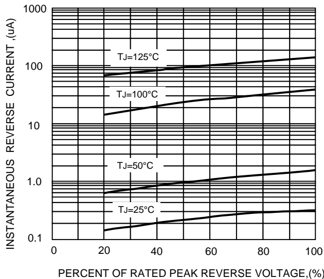
FIG.5-TYPICAL REVERSE CHARACTERISTICS
