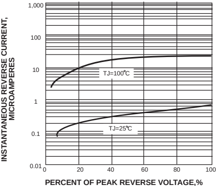
FIG. 4-TYPICAL REVERSE CHARACTERISTICS
