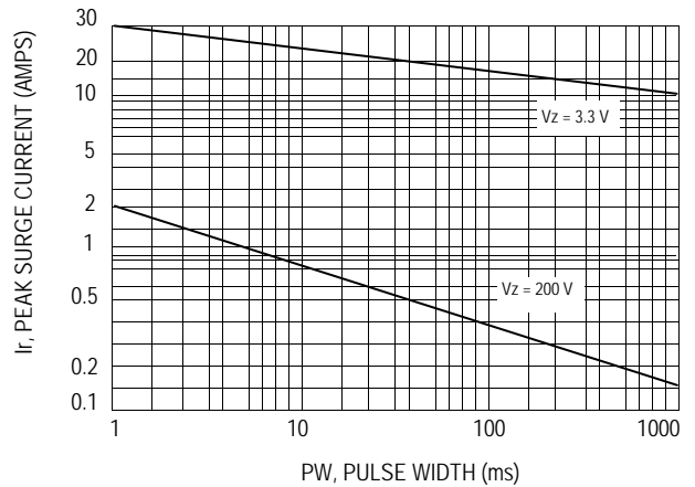
Fig. 3 Peak Surg Current versus Pulse Width
