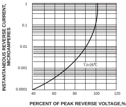
FIG. 2-REVERSE CURRENT VERSUS CONTINUOUS REVERSE VOLTAGE (TYPICAL VALUES)
