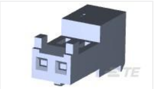
TE Part #3-644020-2 02P MTA100 CONN ASSY 30AU
