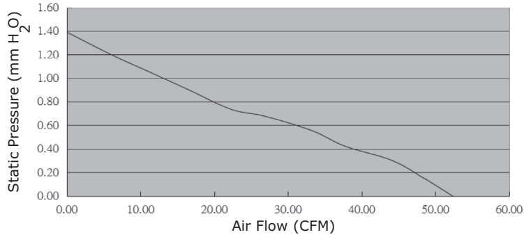
CFM-A225B-015-287
