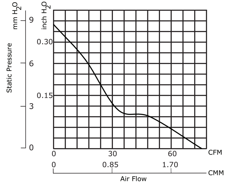
CFM-9225V-345-460
