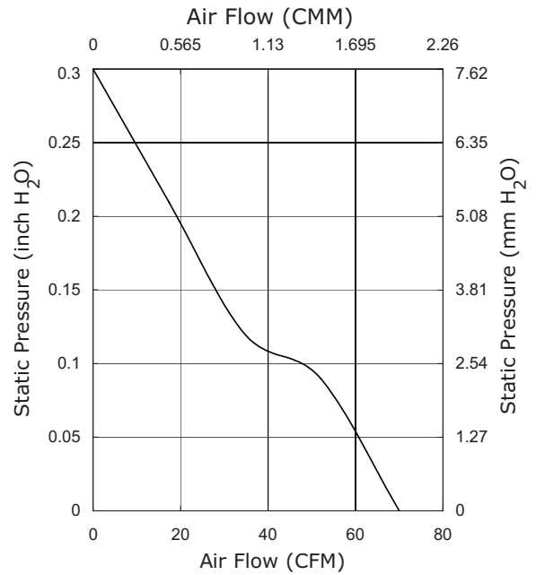
CFM-9225V-142-437
