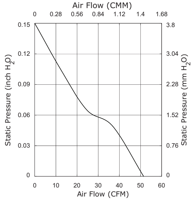
CFM-9225V-242-440
