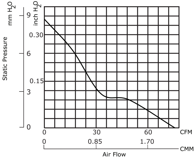
CFM-9225V-245-460
