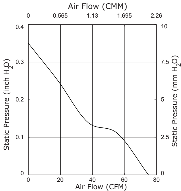
CFM-9225V-145-455
