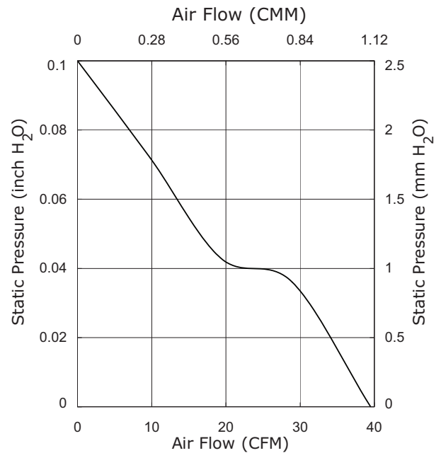
CFM-9225V-224-280
