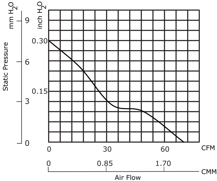
CFM-9225V-342-440
