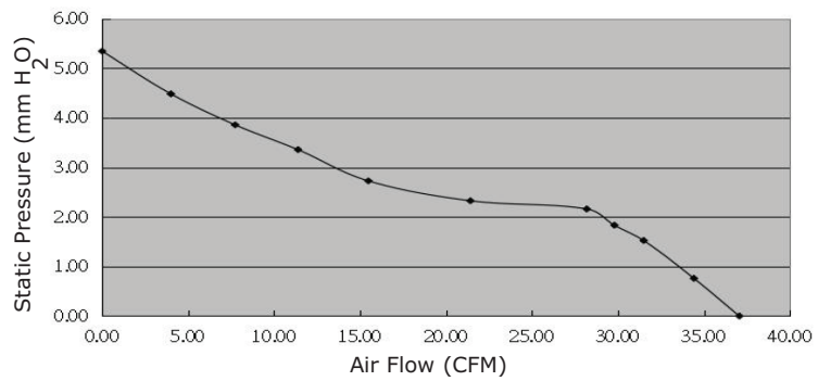
CFM-8038S-250-498
