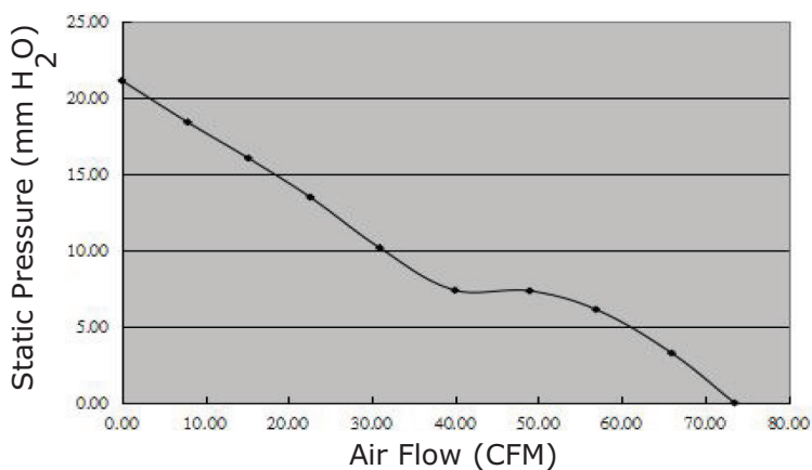
CFM-8025BG68-270-524
