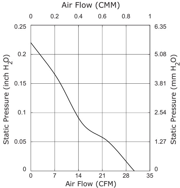
CFM-6015V-254-362
