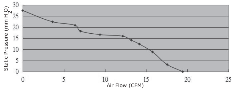
CFM-4020BG-1165-498
