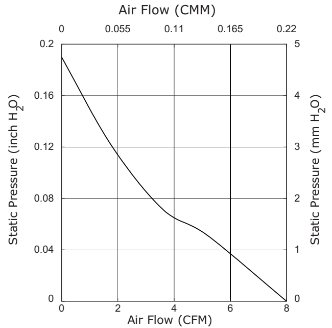
CFM-4010V-070-273
