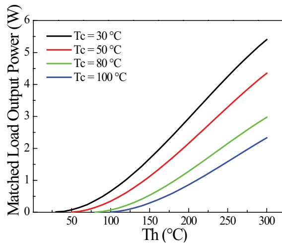
Matched Load Output Power Vs. Th
