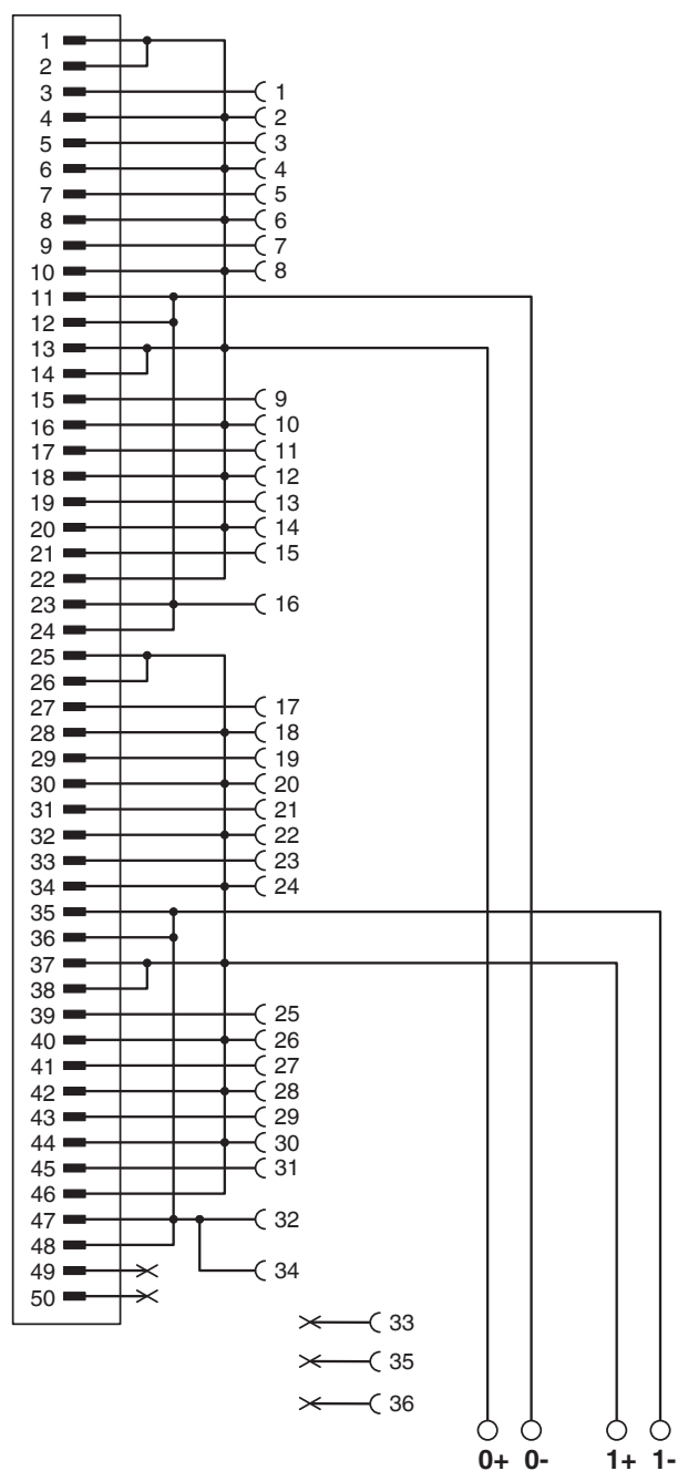
Circuit diagram
